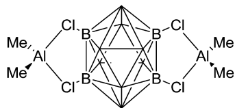
Fig. 10 The ion-like (\text{Me}_2\text{Al})_2\text{B}_{12}\text{Cl}_{12} salt. 87 For clarity, all BCl moieties of the perchlorinated closio -dodecaborate that feature no contact to the [\text{Me}_2\text{Al}]^+ cation have been omitted.
