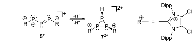
Scheme 2 Reversible protonation/deprotonation reaction between 5^+ and 7^{2+} .
