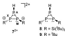
Fig. 2 Substituent arrangement in cyclo -triphosphaphanes 7^{2+} , 8 and 9 .
