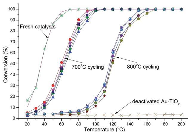
Fig. 5 Light-off curves for catalysts with 5% Au-RANR and commercial Au- \text{TiO}_2 catalyst after multiple 700 and 800\text{ }^\circ\text{C} heating cycles (10 cycles in total).
