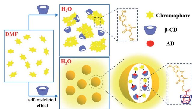
Fig. 1 Concept of emission enhancement of GFP chromophore in aggregated state. Upper: the aggregated emission of GFP chromophore (HB1H1) is very dim due to free conformational motion and ACQ; below: the aggregated emission is greatly enhanced via self-restricted effect and host–guest interaction.
