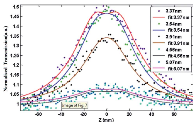
Fig. 11 OA Z-scan of Au–CdSe of different sizes and excitation intensities I_0 = 118 \text{ } \mu\text{J} . 101
