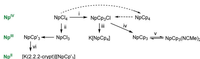
Scheme 1 Synthetic routes to neptunium complexes presented in this work. NpCp 3 is obtained by reduction from NpCp 3 Cl and readily forms the MeCN stabilised solvate. The silylated analogue NpCp' 3 ( \text{Cp}' = \text{C}_5\text{H}_4\text{SiMe}_3 ) is better obtained from the reaction of \text{NpCl}_3 with \text{KCp}' and can be reduced to its K salt. Dotted lines indicate literature procedures. Key: (i) excess \text{KCp} , PhMe; (ii) Na/Hg, \text{Et}_2\text{O} , -\text{NaCl} ; (iii) \text{KCp} , -\text{KCl} ; (iv) Na/Hg, \text{Et}_2\text{O} , -\text{NaCl} ; (v) excess MeCN; (vi) \text{KCl} , 2.2.2-cryptand, THF/ \text{Et}_2\text{O} , -8^\circ\text{C} .
