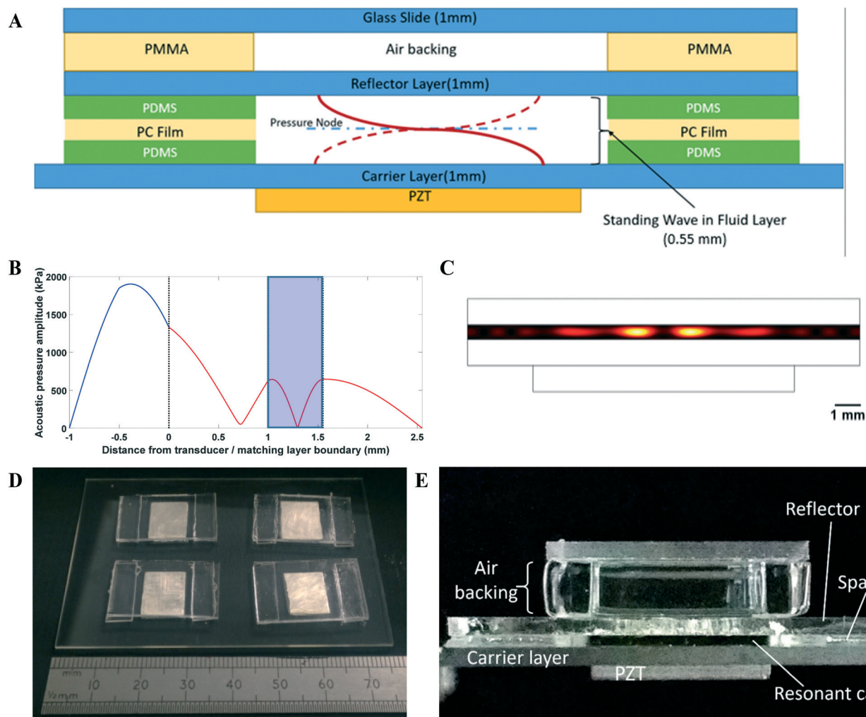
Fig. 1 Bioreactor design and modelling. (A) Schematic diagram detailing resonator design and the dimensions of each layer. (B) A 1-dimensional model was used to confirm cavity resonance frequency and the presence of a pressure node near the centre of the fluid cavity (blue region) for the desired resonator configuration. (C) The transfer impedance model was further validated with a FE model to determine the kinetic energy distribution at resonance, in order to better predict the energy distribution within the pressure node and where the cells are likely to levitate. (D) Angled top view of assembled plate to detail arrangement of multiple resonators on a single double-width glass slide. (E) Side view of assembled resonator, labelled to indicate position of PZT, spacers, carrier and reflector layers. The open sides of the resonant cavity allow for medium exchange within the cavity and alleviate problems with bubble formation experienced with previous closed resonator designs.
