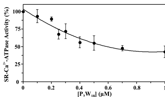
Fig. 3 Inhibition of \text{Ca}^{2+} -ATPase activity by \text{P}_2\text{W}_{18} . \text{Ca}^{2+} -ATPase was determined spectrophotometrically at 340 nm and 25 °C, using the coupled enzyme pyruvate kinase/lactate dehydrogenase assay. The experiments were initiated by the addition of 10 \mu\text{g mL}^{-1} \text{Ca}^{2+} -ATPase, in the presence or absence of 4% (w/w) of the calcium ionophore calcimycin. Data are plotted as means \pm SD and fit to the equation y = 73.126x^2 - 133.62x + 103.45 ( R^2 = 0.9424 ).
