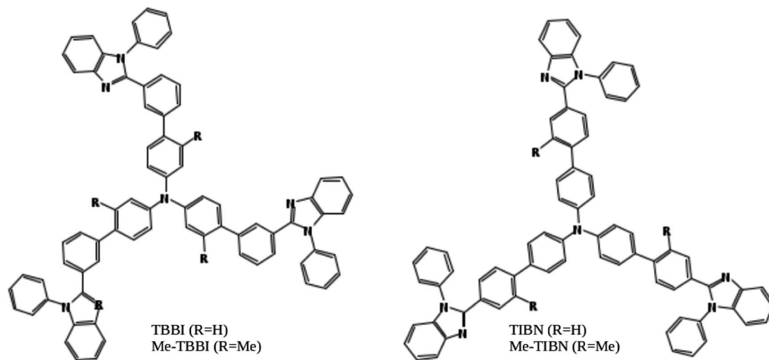
Fig. 1 Chemical structures of the molecules explored in this study. TBBI: tris(3'-(1-phenyl-1 H -benzimidazole-2-yl)biphenyl-4-yl)amine, Me-TBBI: tris(2-methyl-3'-(1-phenyl-1 H -benzimidazole-2-yl)biphenyl-4-yl)amine, TIBN: tris(4'-(1-phenyl-1 H -benzimidazole-2-yl)biphenyl-4-yl)amine, and Me-TIBN: tris(2'-methyl-4'-(1-phenyl-1 H -benzimidazole-2-yl)biphenyl-4-yl)amine.
