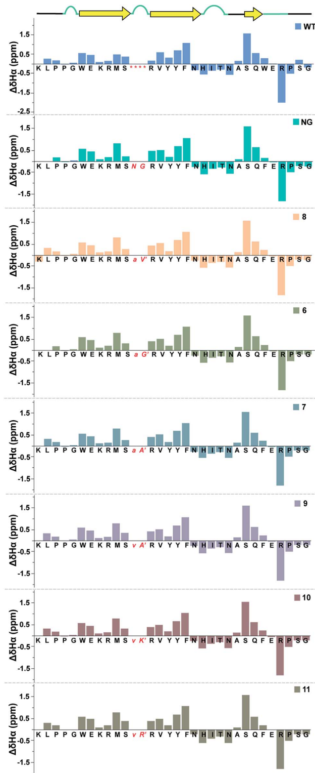
Fig. 7 Comparison of backbone H^{\alpha} chemical shift deviation of the apo-Pin 1 WW domain ( WT ) with the \beta I' turn ( NG ) and the re-engineered Pin 1 variants deduced from the predicted random coil values, 37 indicating minimal perturbation in the secondary structure. The -RSSG- motif in loop 1 of WT is indicated by an asterisk.
