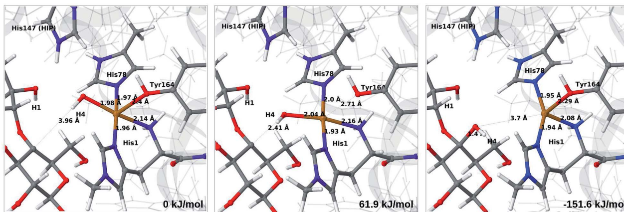
Fig. 13 Reactant 7a (left), transition state (middle) and product 8a (right) for the 7a → 8a reaction with His147 is in the HIP state. The structures were optimised with TPSS/def2-SV(P) and energies were obtained with TPSS-D3/def2-TZVPP.
