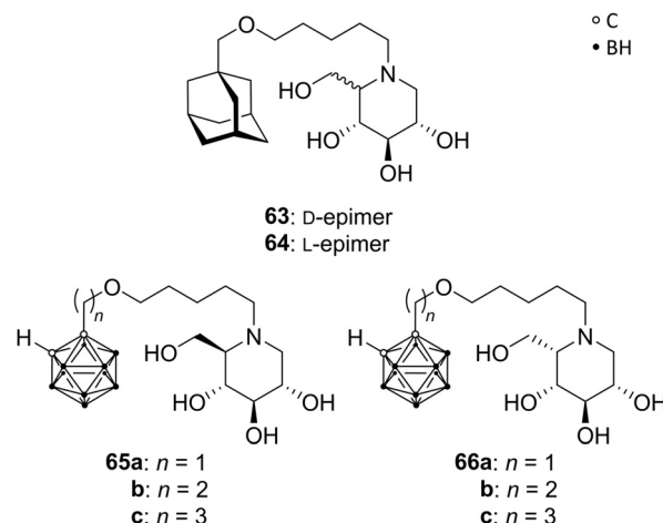
Fig. 17 Structures of AMP-DNMs 63 and 64 and carborane-based analogues 65a-c and 66a-c .
