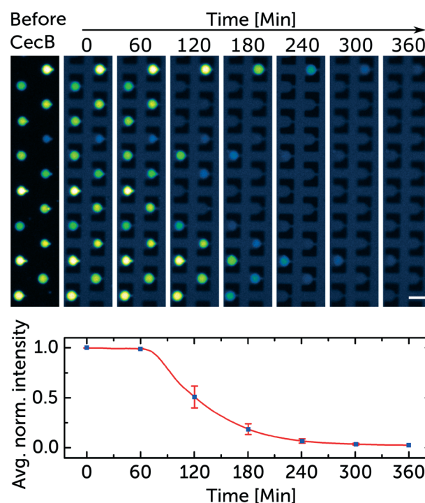
Fig. 3 Representative sample of the data used to quantify the membranolytic activity of cecropin B. Fluorescence microscopy images of trapped GUVTs (DOPC/DOPG lipids mixed at a 3 : 1 ratio). The trapped vesicles encapsulate the membrane impermeable dye HPTS ( 50 \mu\text{M} ). The collage is a subset of images taken every hour displaying the time-dependent membranolytic effect of 5 \mu\text{M} cecropin B on the membrane integrity of the vesicles. The dark blue background marks the arrival of the peptide to the chamber. The averaged normalised fluorescence decrease in intensity from the 14 trapped vesicles is mapped. The means and standard error bars correspond to the fluorescence intensity of all the vesicles in the aligned frames in the collage. Scale bar represents 50 \mu\text{m} . The corresponding video is in the ESI† SV1.
