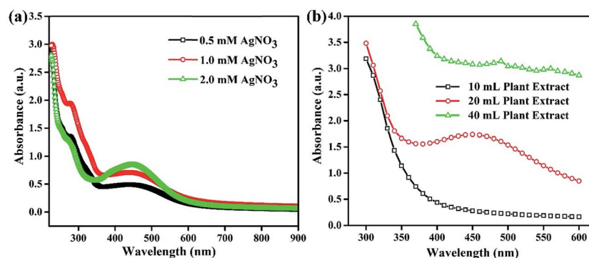
Fig. 2 UV-vis absorption spectra of Ag NPs synthesized at different concentrations of (a) \text{AgNO}_3 and (b) the plant extract.
