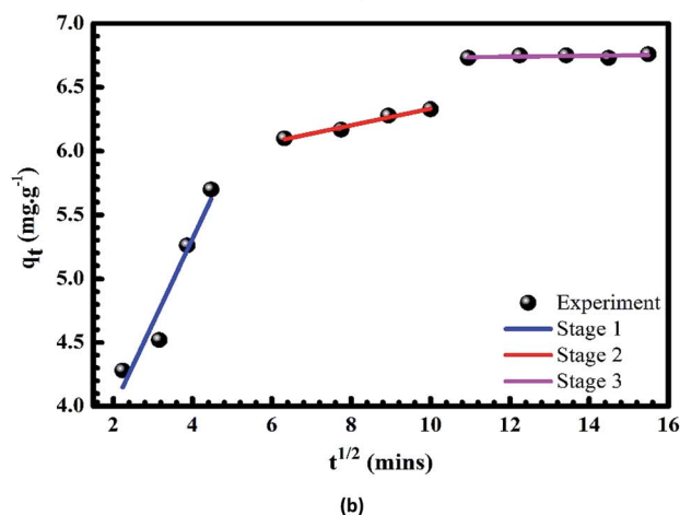
Fig. 11 Plots of intra-particle diffusion models of the adsorption of \text{Cr(III)} (a) and MB (b) onto pomelo fruit peel.
