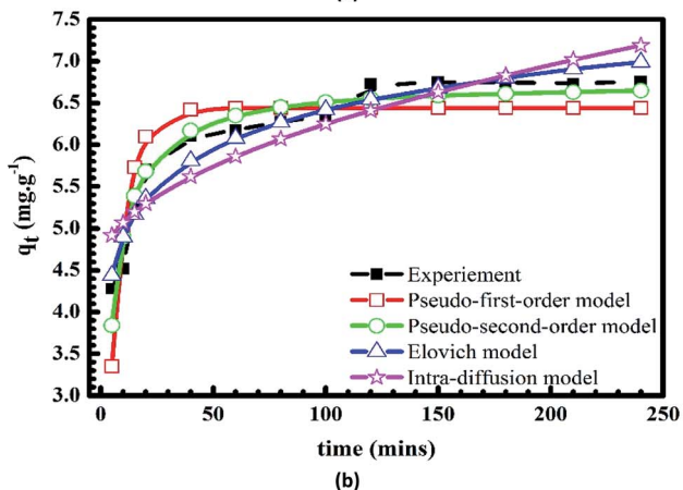
Fig. 10 Plots of kinetic models of the adsorption of MB (a) and \text{Cr(III)} (b) onto pomelo fruit peel.
