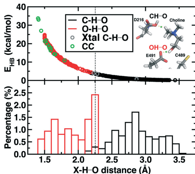
Fig. 9 (top) Hydrogen bond energy ( E_{HB} , in kcal mol −1 ) versus X–H \cdots O distance for i) snapshot MD distances with X=O (red circles), X=C (black circles), ii) all observed close contacts in crystal structures (CC, green circles), and the X=C non-covalent interactions observed in CutC (Xtal C–H \cdots O, gray circles). A snapshot showing the C–H \cdots O and O–H \cdots O hydrogen bond is provided in inset with the BCP shown as a green sphere. (bottom) Normalized distribution of CH \cdots O and OH \cdots O distances from MD snapshots as described for the top pane. A qualitative cutoff between CH \cdots O and OH \cdots O distances is indicated by a vertical dashed line at 2.25 Å.
