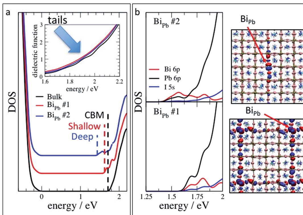
Fig. 9 Results of theoretical calculations. (a) Density of state of the bulk (black) and two neutral Bi Pb defect configurations corresponding to shallow (red) and deep (blue) defect states. The zero of the energy axis is set to the valence band maximum (VBM). The lowest (half-filled) energy defect state of the first configuration overlaps with the bulk CBM. On the contrary, the corresponding state of the second configuration is well separated from the conduction band. In the inset it is reported the low energy part of the absorption spectrum, which shows the defect related low energy tails. (b) Contribution of Bi 6p, Pb 6p and I 5s atomic orbitals to the DOS in the energy range of defect states. On the right-hand side of the panel are reported the isosurface of the defect states of minimum energy. Isosurfaces are colored in blue and red according to the sign of the corresponding orbitals to put in evidence their antibonding character.
