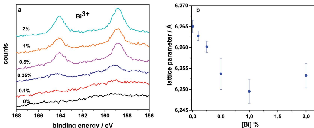
Fig. 8 Structural characterization of perovskite films containing Bi (a) XPS spectra showing the characteristic signal for Bi 3+ which increases for higher Bi content. (b) Lattice parameter deduced from fitting XRD spectra. Incorporation of Bi decreases the lattice parameter.
