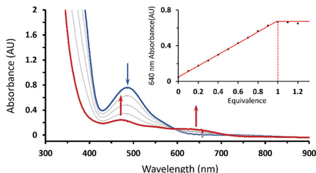
Fig. 1 UV-vis spectral changes of the reaction of 1 (1.0 mM, blue trace) with 1 equiv. of HOTf in THF at -90^\circ C . Inset: Titration curve of 1 with HOTf. X-axis: the equivalents of HOTf, Y-axis: the conversion ratio of the absorption peak at 640 nm.
