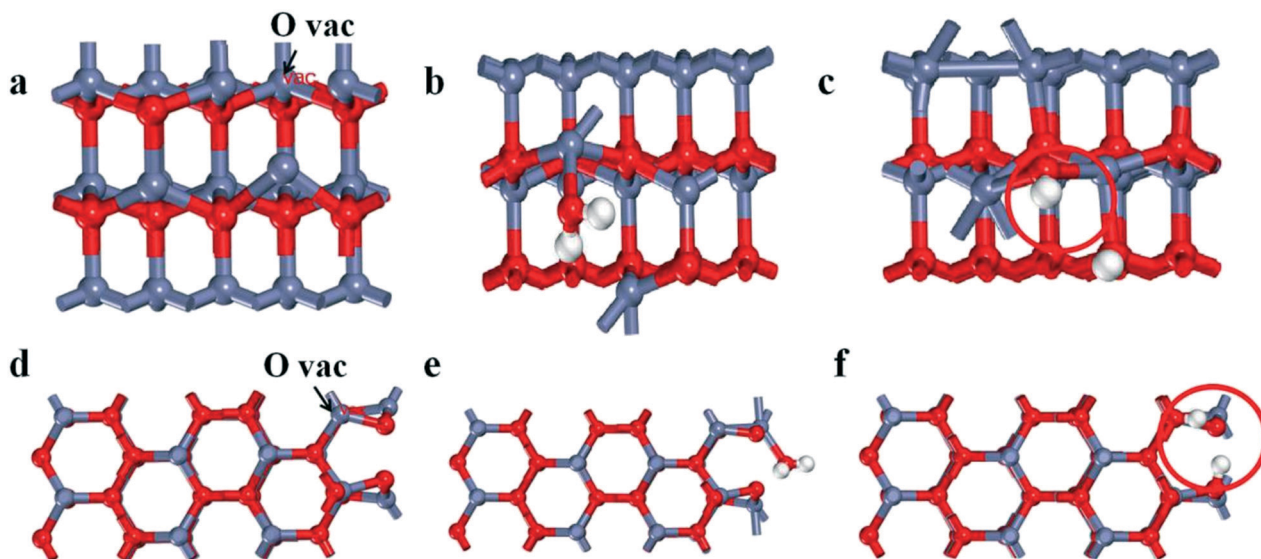
Fig. 3 Side views of the surface structures of defective ZnO (a) with O vacancies, (b) adsorption and (c) dissociation \text{H}_2\text{O} on the (100) plane, side views of the surface structures of defective ZnO (d) with O vacancies and (e) adsorption and (f) dissociation \text{H}_2\text{O} on the (101) plane.
