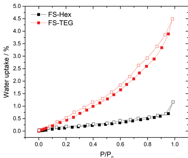
Fig. 3 Water vapor isotherms of FS-Hex and FS-TEG at 20.0^\circ\text{C} and up to 23 mbar.
