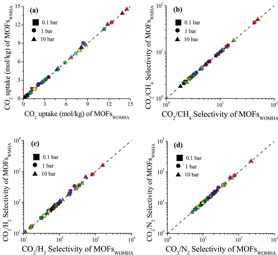
Fig. 3 Comparisons of the (a) single-component CO 2 uptakes and selectivities for the (b) CO 2 /CH 4 : 50/50, (c) CO 2 /H 2 : 15/85, and (d) CO 2 /N 2 : 15/85 separation performances of MOFs with missing hydrogen atoms (MOF WMHA ) and without missing hydrogen atoms (MOF WOMHA ).
