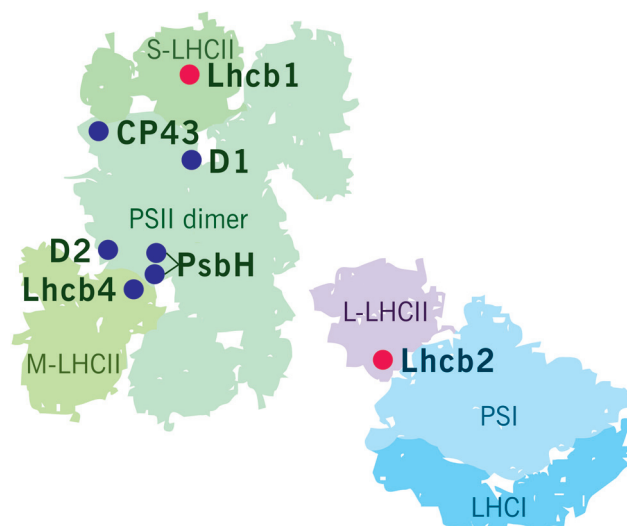
Fig. 4 STN7 and STN8 dependent phosphosites in PSII–LHCII supercomplex and in PSI–LHCI–LHCII supercomplex. Main targets of the STN7 kinase are marked with red dots and those of the STN8 kinase with blue dots.
