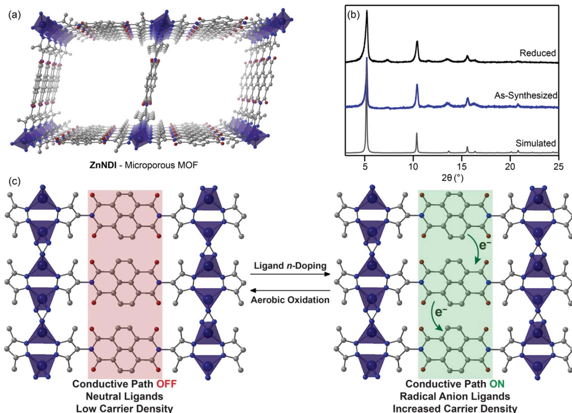
Fig. 1 (a) Structure of the microporous MOF ZnNDI; (b) PXRD data demonstrating that the MOF structure remains intact after ligand reduction; (c) the ordered stacks of NDI ligands undergo reversible reduction to their radical anion form, creating a through-space charge transport pathway via NDI hopping that results in increased electrical conductivity.
