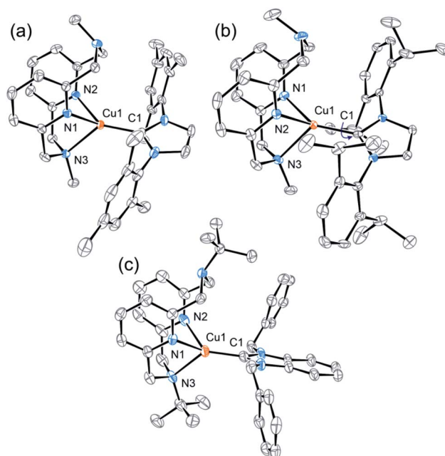
Fig. 2 ORTEP of 1 (a), 2 (b), and 3b (c) at 50% probability level according to XRD data. Anions, solvent molecules, and hydrogen atoms are omitted for clarity. In the case of 2 , the structure was inverted for clarity. The structures of 3c and 3d are present in ESI † .
