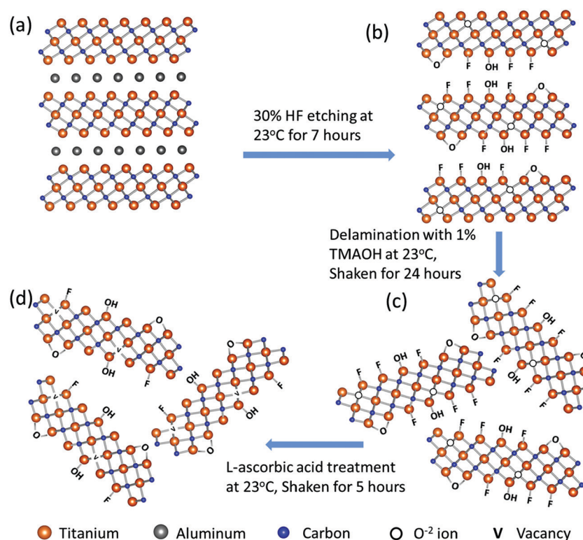
Fig. 1 Schematic diagram of r\text{-Ti}_3\text{C}_2\text{T}_x synthesis.
