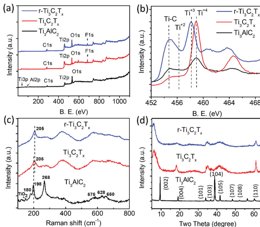
Fig. 3 (a) XPS survey spectra, (b) high resolution XPS spectra of Ti 2 p region, (c) Raman spectra, and (d) XRD patterns, respectively, of Ti 3 AlC 2 MAX phase (black), Ti 3 C 2 T x (red), and r-Ti 3 C 2 T x (blue).
