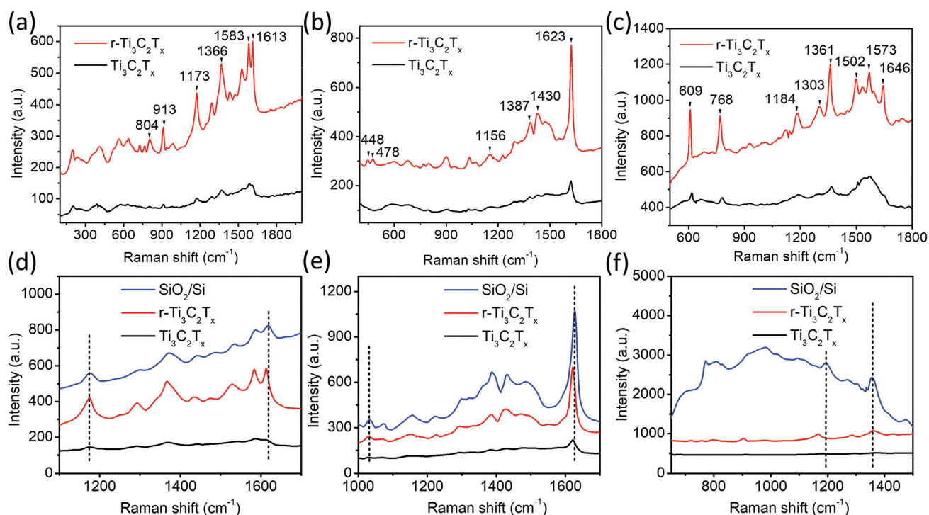
Fig. 6 SERS spectra of (a and d) CV, (b and e) MB, and (c and f) R6G collected on \text{Ti}_3\text{C}_2\text{T}_x/\text{SiO}_2/\text{Si} (black) and \text{r-Ti}_3\text{C}_2\text{T}_x/\text{SiO}_2/\text{Si} (red), and bare \text{SiO}_2/\text{Si} (blue) substrates. Concentration of dyes on \text{SiO}_2/\text{Si} substrate is 1 M in water.
