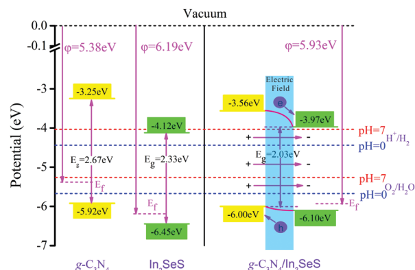
Fig. 6 Potential of band-edge positions for \text{g-C}_3\text{N}_4 , monolayer \text{In}_2\text{SeS} and the \text{In}_2\text{SeS}/\text{g-C}_3\text{N}_4 heterostructure.
