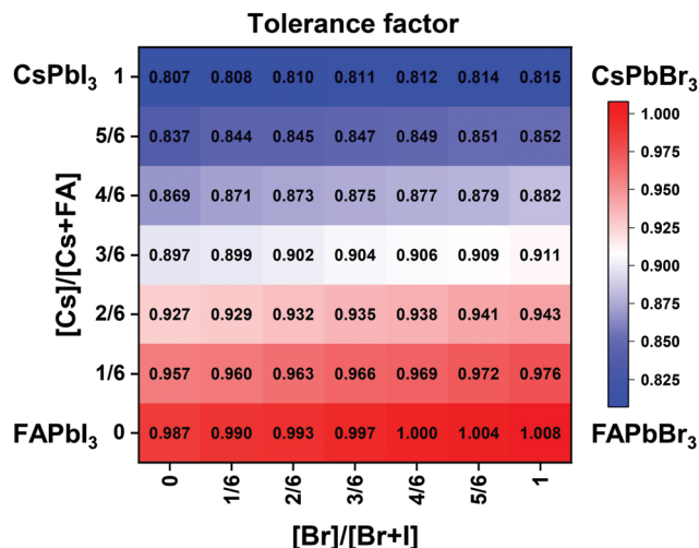
Fig. 2 Effective tolerance factor map for the \text{Cs}_x\text{FA}_{1-x}\text{Pb}(\text{Br}_{y1-y})_3 compositional space tuned via composition engineering.
