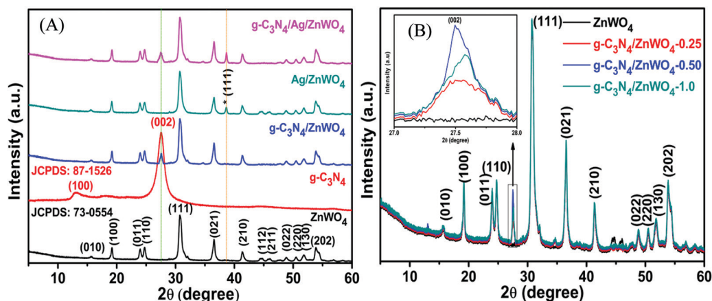
Fig. 2 Powder XRD of (A) pure monoclinic primitive ZnWO 4 and the composites of ZnWO 4 with g-C 3 N 4 and Ag(0) and (B) composites with varying amounts of g-C 3 N 4 .
