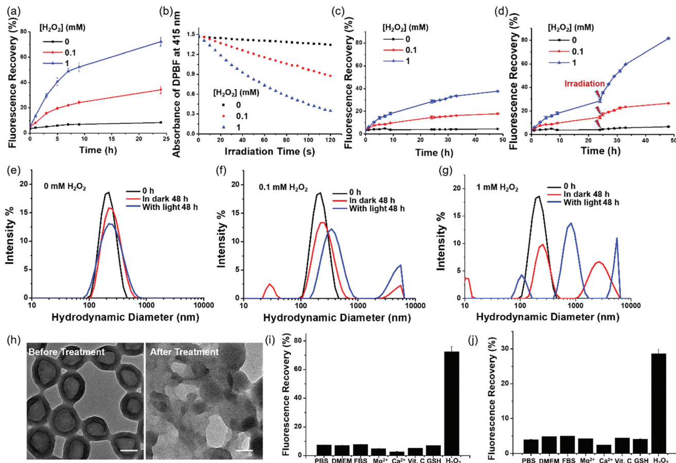
Fig. 3 (a) Recovery of Pc fluorescence ( \lambda_{\text{ex}} = 610 \text{ nm} , \lambda_{\text{em}} = 707 \text{ nm} ) upon exposure of PDA-Dox-Pc-QRH to different concentrations of \text{H}_2\text{O}_2 . (b) Comparison of the rates of decay of DPBF sensitised by PDA-Dox-Pc-QRH after being treated with different concentrations of \text{H}_2\text{O}_2 for 24 h. Recovery of Dox fluorescence ( \lambda_{\text{ex}} = 488 \text{ nm} , \lambda_{\text{em}} = 550 \text{ nm} ) upon exposure of PDA-Dox-Pc-QRH to different concentrations of \text{H}_2\text{O}_2 (c) without and (d) with light irradiation ( \lambda > 610 \text{ nm} ) for 20 min at 24 h post-treatment with \text{H}_2\text{O}_2 . Change in hydrodynamic diameter distribution of PDA-Dox-Pc-QRH (e) without and with treatment with (f) 0.1 and (g) 1 mM of \text{H}_2\text{O}_2 for 48 h. Light irradiation ( \lambda > 610 \text{ nm} ) was applied for 20 min at 24 h post-treatment with \text{H}_2\text{O}_2 . (h) TEM images of PDA-Dox-Pc-QRH before and after treatment with 1 mM of \text{H}_2\text{O}_2 for 48 h with light irradiation as above. Scale bars: 100 nm. Recovery of (i) Pc and (j) Dox fluorescence for PDA-Dox-Pc-QRH in PBS, DMEM or FBS with 0.5% Tween 20 at 37^\circ\text{C} for 24 h, and after treatment with different species at a concentration of 1 mM in PBS with 0.5% Tween 20 at 37^\circ\text{C} for 24 h. Data are reported as the mean \pm SD of three independent experiments. For figure (a) to (g), the measurements were performed in PBS with 0.5% Tween 20 at 37^\circ\text{C} . The concentration of the NPs was fixed at [\text{Pc}] = 2.0 \mu\text{M} or [\text{Dox}] = 1.8 \mu\text{M} .
