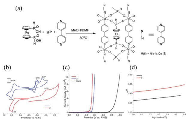
Fig. 2 Co II /Ni II -Fe II bimetallic coordination polymers as a H 2 evolution electrocatalyst: (a) synthesis scheme, (b) CV curves in MeCN containing 0.1 M Bu 4 NBF 4 with a sample-modified glassy carbon electrode, (c) LSV curves in 0.5 M H 2 SO 4 at a scan rate of 0.05 V s -1 , and (d) their corresponding Tafel plots. Adapted from ref. 70 with permission from The Royal Society of Chemistry.
