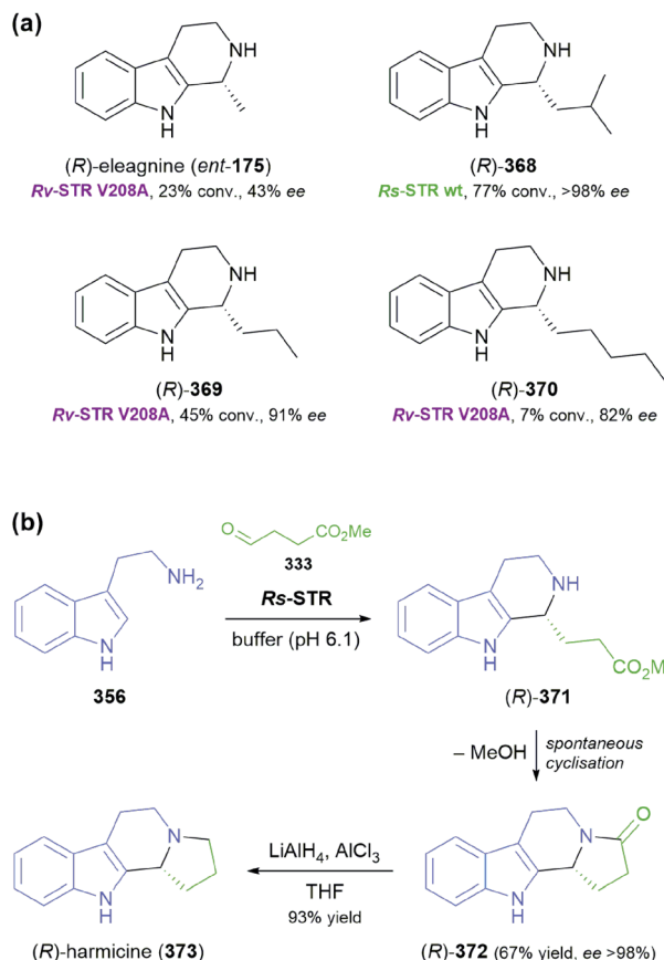
Scheme 47 (R)-Selective Pictet–Spengler reactions of strictosidine synthases (STRs): (a) 1-alkyl-tetrahydro- \beta -carbolines obtained from tryptamine (356) and small, aliphatic aldehydes, (b) two-step chemo-enzymatic synthesis of (R)-harmicine (373).
