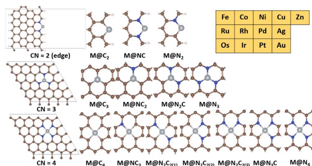
Fig. 2 Calculation models for \text{M}@\text{N}_x\text{C}_y catalysts. Grey, brown, blue and white balls represent transition metal, carbon, nitrogen and hydrogen atoms, respectively. The 13 late transition metals considered in this study are shown as a table.
