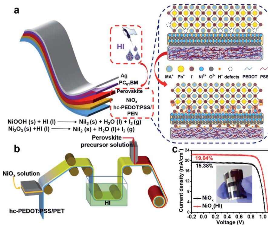
Fig. 1 In situ bifacial passivation mechanism and device preparation. (a) Diagram of the passivation mechanism. (b) Fabrication procedure for perovskite solar cells by R2R process. (c) J - V curves of flexible devices ( 1.01 \text{ cm}^2 ) with and without HI treatment. Inset presents the photograph of flexible perovskite solar cells.
