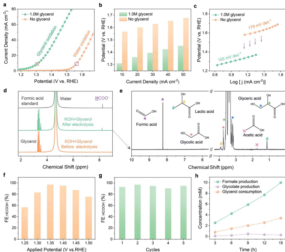
Fig. 2 Glycerol electrooxidation performance. (a) Linear sweep voltammetry (LSV) plots (all LSV plots were collected with a scan rate of 5 \text{ mV s}^{-1} in \text{N}_2 -saturated electrolyte with no I-R compensation). (b) Input potentials at various current densities. (c) Tafel slopes for the OER and glycerol oxidation in 1.0 \text{ M KOH} solution both with and without 1.0 \text{ M} glycerol. Purple arrows inset indicate the significant potential decrease at various current densities when 1.0 \text{ M} glycerol is added. (d) ^1\text{H} NMR spectra of the formic acid standard and electrolytes ( 1.0 \text{ M KOH} + 1.0 \text{ M glycerol} ) before and after 12 \text{ h} of electrolysis at 1.35 \text{ V} vs. RHE. Due to the higher initial glycerol concentration, the intensity of ^1\text{H} NMR peaks for glycerol did not decrease significantly after electrolysis. (e) High-resolution ^1\text{H} NMR spectra (water peak was removed from 4 to 6 \text{ ppm} ) of the 1.0 \text{ M KOH} + 1.0 \text{ M glycerol} solution after 12 \text{ h} of electrolysis (the symbols on the top of the peaks represent each type of proton present). (f) Faradaic efficiencies of formic acid at various potentials (each potential underwent 12 \text{ h} of electrolysis). (g) Faradaic efficiencies of formic acid for five successive electrolysis cycles at 1.35 \text{ V} vs. RHE. (h) Concentration changes of the reactant (glycerol), main product (formic acid), and representative intermediate species (glycolic acid) with electrolysis time.
