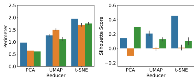
Fig. 5 Comparison of the overall classification results for PCA, UMAP and t-SNE, based on average P - and S scores, applied to: numerical data (blue), image data (orange); and feature extractor output (green).
