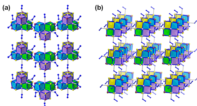
Fig. 7 Arrangement of the \text{N}_2\text{H}_4 -linked [\text{Mn}_6(\mu_6\text{-S})(\text{AsS}_3)_4]^{2-} clusters (a) in 2\text{D}-\{[\text{Mn}_6(\mu_6\text{-S})(\text{N}_2\text{H}_4)_2(\mu\text{-N}_2\text{H}_4)_2(\mu_3\text{-AsS}_3)_4]^{2-}\} and (b) in 3\text{D}-\{[\text{Mn}_6(\mu_6\text{-S})(\mu\text{-N}_2\text{H}_4)_3(\mu_3\text{-AsS}_3)_4]^{2-}\} . Counterions are omitted for clarity. Color code: As-plum, Mn-lavender, S-yellow, N-blue.
