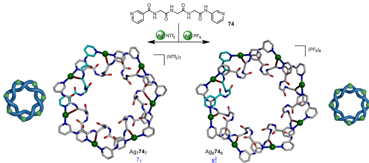
Fig. 26 Anion-mediated synthesis of 7_1 metallaknot \text{Ag}_7\mathbf{74}_7 or 8_1^2 metallaknot \text{Ag}_8\mathbf{74}_8 by coordination of \text{Ag}^+ ions to pyridyl-capped polypeptide ligand \mathbf{74} . 103
