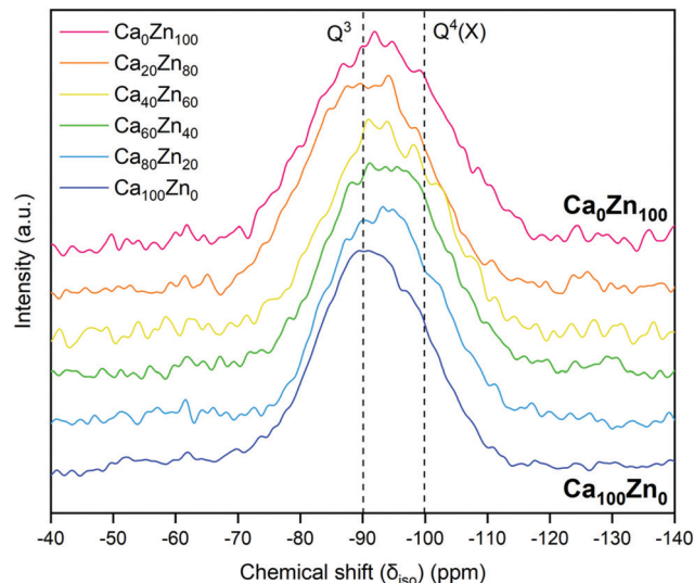
Fig. 8 ^{29}\text{Si} MAS NMR spectra for the \text{Ca}_x\text{Zn}_y glass series overlaid with chemical shifts approximately representative of \text{Q}^3 and \text{Q}^4(\text{X}) (where X is a network former other than Si) species. Indicative location of \text{Q}^3 and \text{Q}^4(\text{X}) species are shown.
