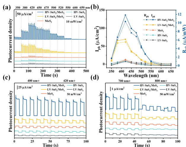
Fig. 6 (a) The amperometric I - t curves irradiated by light at different wavelengths. (b) I_{ph} and R_{ph} as a function of wavelength. (c) The amperometric I - t curves irradiated by light in 400+ and 420+ nm. (d) The amperometric I - t curves irradiated by light in 700+ and 800+ nm.
