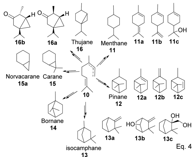
Fig. 3 Products derived from cyclization of allylic cation 10 .
