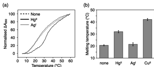
Fig. 4 (a) Melting curves of a DNA duplex containing an \text{Im}^{\text{OC}}\text{-Im}^{\text{OC}} base pair ( 1\cdot2 ) in the presence of \text{Hg}^{\text{II}} and \text{Ag}^{\text{I}} ions. [duplex] = 2.0\text{ }\mu\text{M} , [metal ion]/[duplex] = 0 (dashed line) or 1 (solid lines) in 10 mM HEPES buffer (pH 7.0), 100 mM \text{NaNO}_3 , 0.2\text{ }^{\circ}\text{C min}^{-1} . (b) Melting temperatures. N = 3 . The error bars represent the standard errors. The melting temperature in the same buffer in the presence of \text{Cu}^{\text{II}} is also shown.
