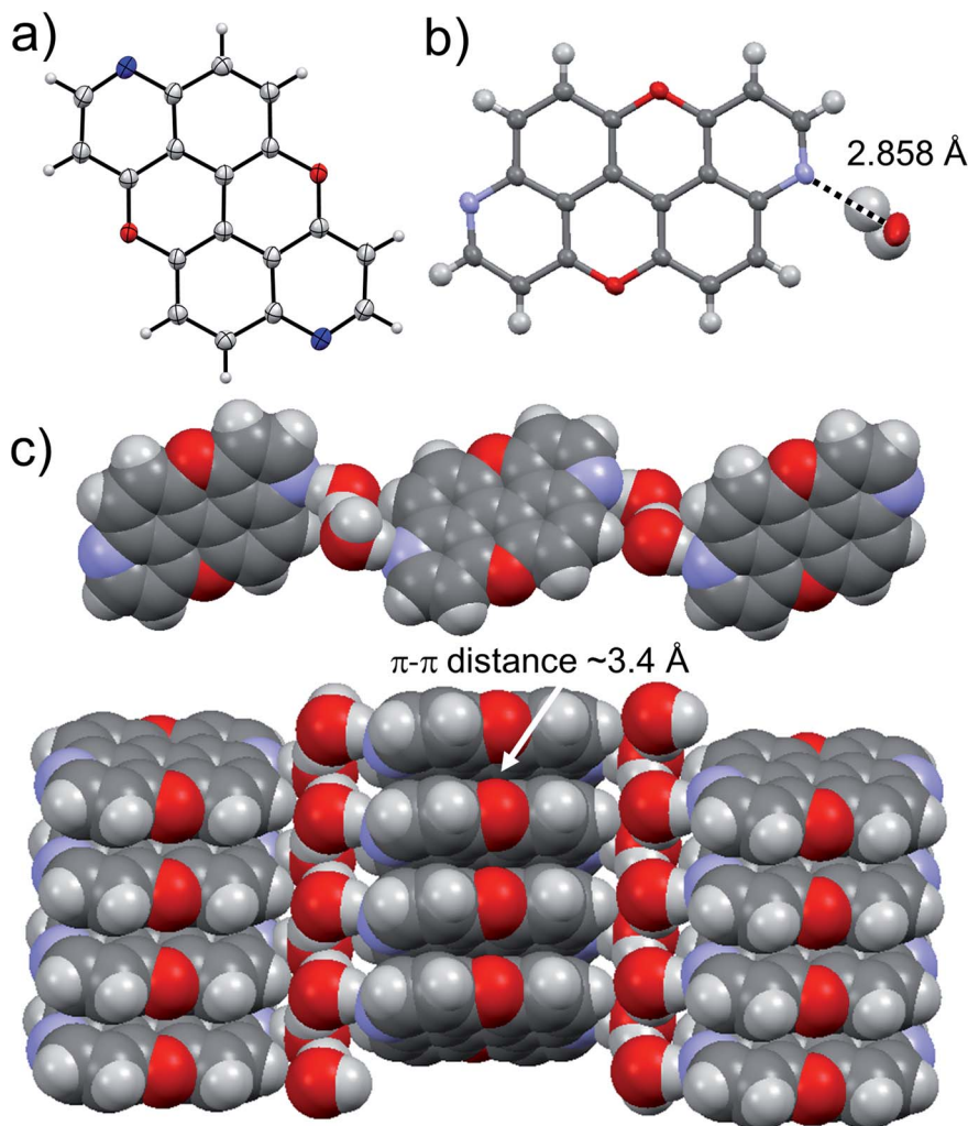
Fig. 9 Single-crystal X-ray structure of 3,9-N,N-PXX . ORTEP representation (a) and structure of the water and 3,9-N,N-PXX molecules engaging into H-bonds (b) depicting the supramolecular polymer organisation (c). Space groups: P2_1/c . Atom colours: red O, blue N, grey C, white H.
