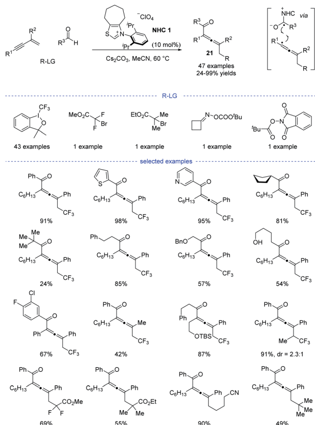
Scheme 18 NHC-catalyzed three-component 1,4-carbofunctionalization of 1,3-enynes.
