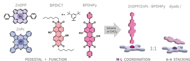
Fig. 1 General scheme of dyad design and components: (left to right) ZnPc and ZnDPP molecular pedestals, the perylene-functional components BPDIC7 and BPDIPy, and the resulting dyad and triads obtained via metal-ligand (M-L) or \pi - \pi associations in a 1:1 or 2:1 ratio.
