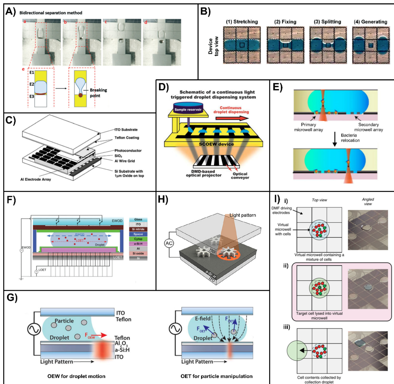
Fig. 2 Magnetic and optical manipulation of samples for DMF. (A) Bidirectional separation of magnetic particles on the EWOD platform using external magnet and sequential electrode activation. Reproduced with permission from ref. 64. Copyright 2020, the Royal Society of Chemistry. (B) "One-to-three" droplet separation where magnetic particles are retained at the center. Reproduced with permission from ref. 50. Copyright 2021, the Royal Society of Chemistry. (C) Schematic structure of a double-sided OEW device with an electrode array. ITO: indium-tin oxide. Reproduced with permission from ref. 66. Copyright 2003 Elsevier. (D) Schematic of the single-sided continuous optoelectrowetting (SCOEW) device. Droplets are manipulated at an arbitrary position on the device surface by an optical projector. Reproduced with permission from ref. 67. Copyright 2010, the Royal Society of Chemistry. (E) Cross-sectional view of bacterial relocation via an optical tweezer in an EWOD droplet. Reproduced with permission from ref. 81. (F) Cross-sectional schematic of a lateral-field OET (LOET) integrated on EWOD platform. Cytop: a hydrophobic coating; a-Si:H: hydrogenated amorphous silicon. Reproduced with permission from ref. 83. Copyright 2009, the Royal Society of Chemistry. (G) Schematic diagram of a unified platform for OEW and an OET, where the OEW force drives the droplet and the OET force manipulates particles within the droplet. Reproduced with permission from ref. 84. Copyright 2011, the Royal Society of Chemistry. (H) Schematic of an OET device with light-driven micro-gears. Reproduced with permission from ref. 86. (I) An EWOD platform with 2D cell culture and laser-induced single cell lysis. From (i) to (iii): the process of the assay, including cell culture in the EWOD chip, selective lysis of the target cell by a laser, and collection of the lysed cell contents. Descriptions of the virtual microwell can be found in Fig. 4A and in section 3.1. Reproduced with permission from ref. 12.
