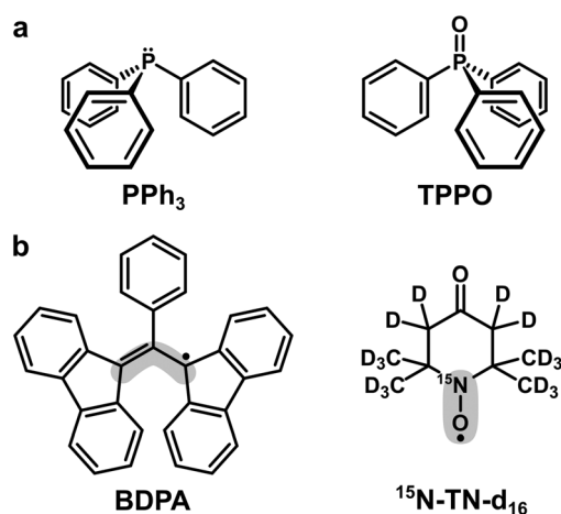
Scheme 1 (a) Trivalent (PPh 3 ) and pentavalent (TPPO) phosphorus compounds used as target molecules. (b) Organic radicals used as PAs. The grey areas mark the sites with the largest electron spin density: ~40% for BDPA and ~90% for 15 N-TN-d 16 . 18
