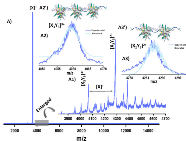
Fig. 5 (A) ESI MS showing the supramolecular adducts in NCA-1.0. (A1) Enlarged view of the same. (A2) The experimental and theoretical isotopic patterns of [X 3 Y 3 ] 3+ . (A2') Schematic representation of [X 3 Y 3 ] 3+ . (A3) The experimental and theoretical isotopic patterns of [X 2 Y 3 ] 2+ . (A3') Schematic representation of [X 2 Y 3 ] 2+ . (X = [Ag 14 (NT) 7 (DPPH) 2 Cl 2 ] + ; Y = DPPH). Color codes: grey, Ag; blue/sea green, C; yellow, S; orange, P; green, Cl; white, H.
