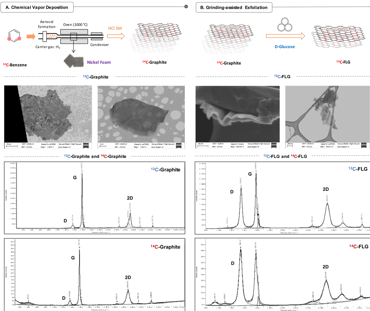
Fig. 2 (A) Synthesis and characterization of 14 C-graphite. Upper panel: schematic representation of the CVD preparation of 14 C-graphite from 14 C-benzene. Middle panel: morphological characterization of 12 C-graphite by STEM. Scale: 10 μm (left) and 1 μm (right). Lower panel: Raman spectra of 12 C-graphite (up) and 14 C-graphite (down). (B) Synthesis and characterization of 14 C-FLG. Upper panel: schematic representation of the grinding-assisted exfoliation of 14 C-graphite to provide 14 C-FLG. Middle panel: morphological characterization of 12 C-FLG by STEM. Scale: 100 nm (left) and 200 nm (right). Lower panel: Raman spectra of 12 C-FLG (up) and 14 C-FLG (down).
