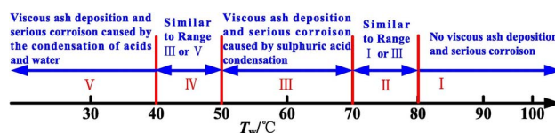
Fig. 8 Ash deposition and corrosion characteristics as a function of wall temperatures. 173
