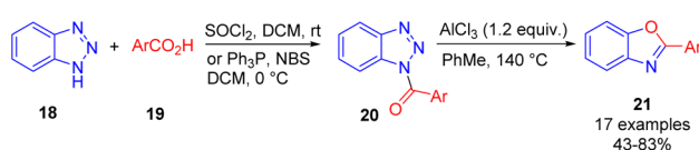
Scheme 14 Synthesis of benzoxazoles from NH-benzotriazoles.
